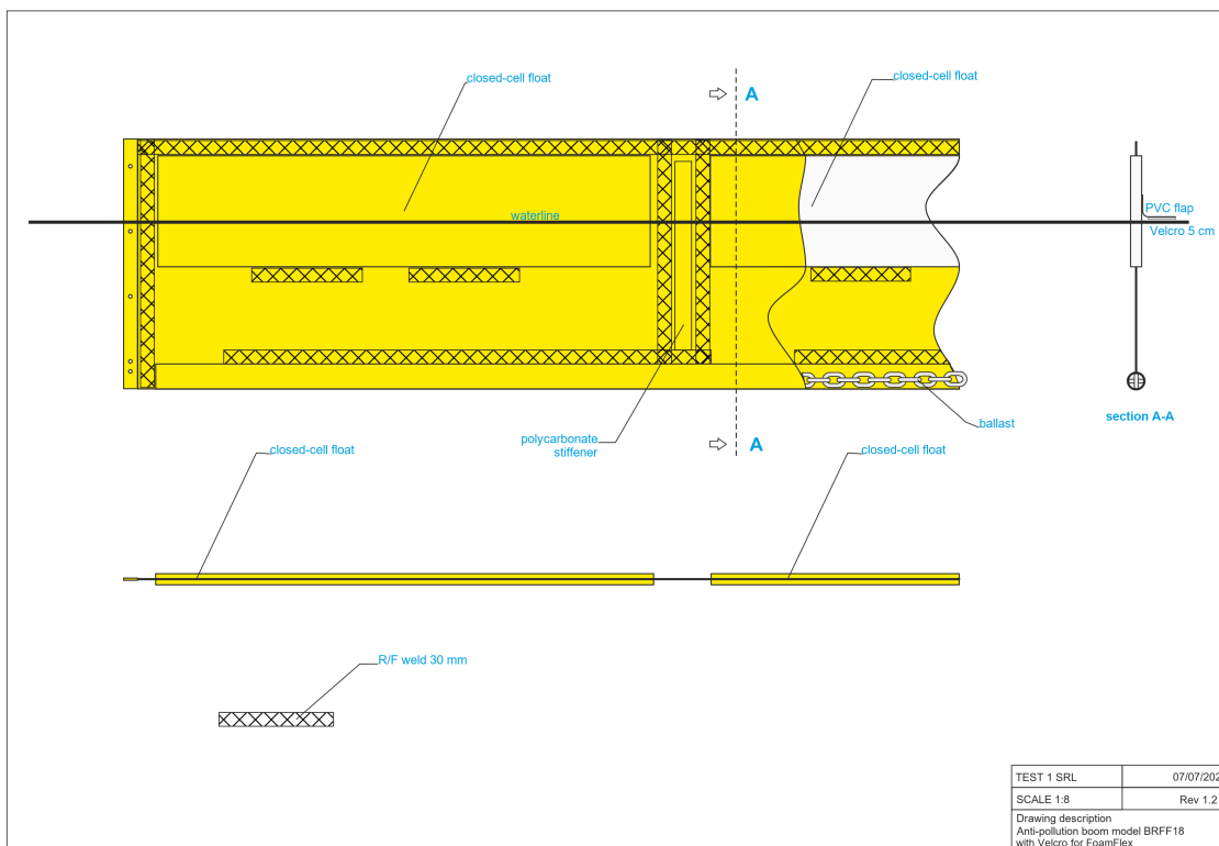
Section A-A - BRFF18 anti-pollution boom model with Velcro for FoamFlex (TEST1 SRL, Rev 1.2, 07/07/2021)
